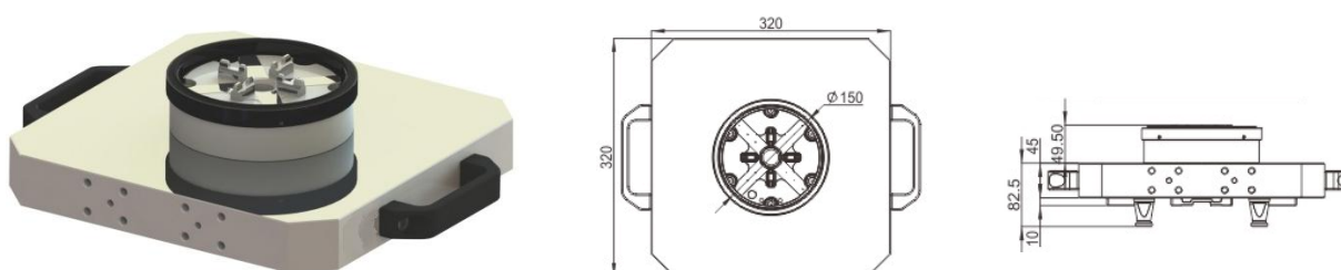
Item No.: EL-UPC0002 UPC holder with pneumatic power chuck, ITS100
