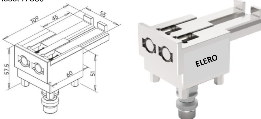
Obj. č.: EL-T0002 Precision toolmaker vise – pendulum, ITS50 With microadjusting in 3axis, clamping range 0-100mm, angle setting 0-360°
