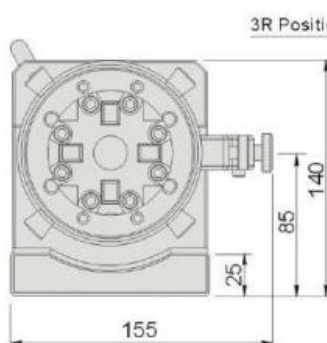
3R Positioning Chuck
