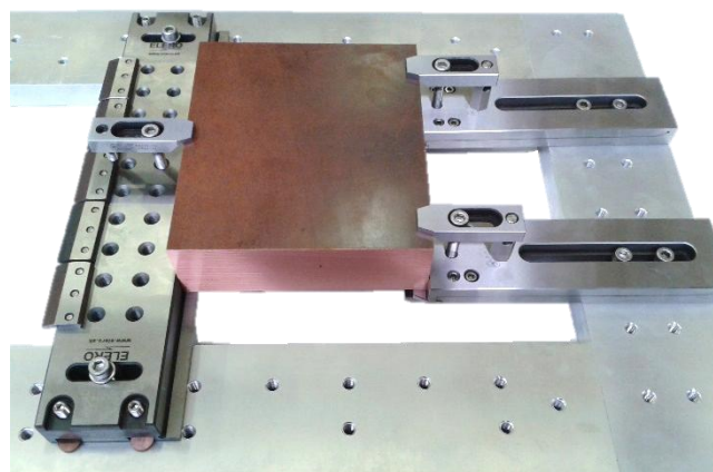
1x DSRSSM8 Double sided ruler stainless steel M8 resp. M6 + 2x MACSS60X220 Adjustable clamp - stainless steel 60x220+5mm, M8, with micro adjusting, clamping in level Z=+5mm
