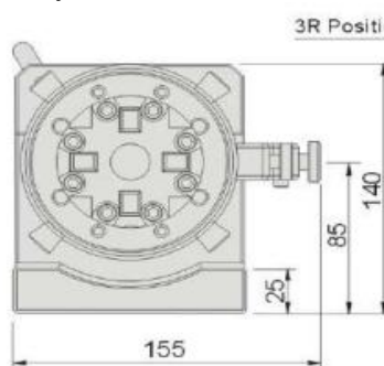
3R Positioning Chuck
