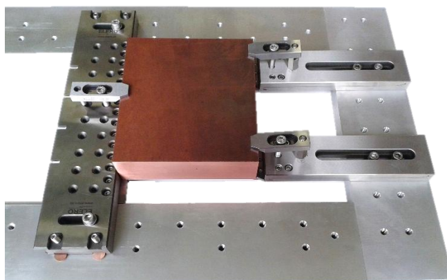
1x DSRSSM8 Double sided ruler stainless steel M8 resp. M6 + 2x MACSS60X220 Adjustable clamp - stainless steel 60x220+5mm, M8, with micro adjusting, clamping in level Z=0mm
