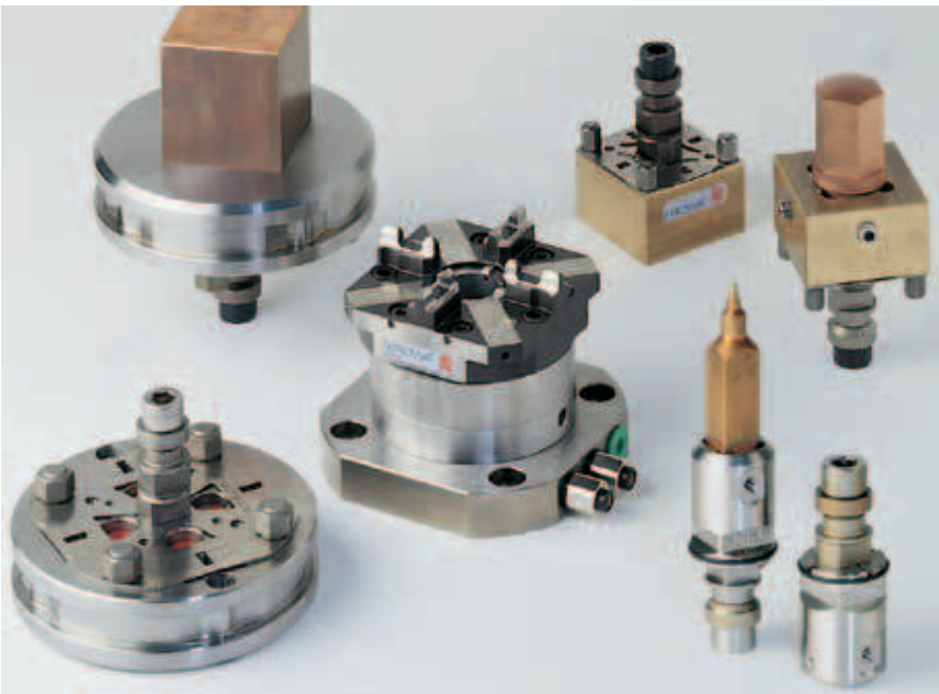
Three pallet sizes - one chuck. EROWA ITS Compact CombiChuck.
